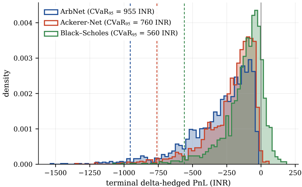
Delta-hedge PnL on 2000 rough-Bergomi paths (30-day horizon)
