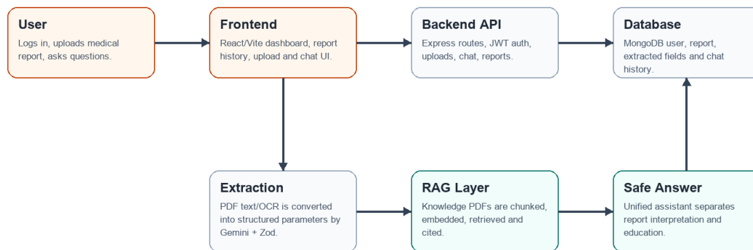
Figure 3.1: The project combines report storage, structured extraction, RAG retrieval and a safety-aware chat layer.
