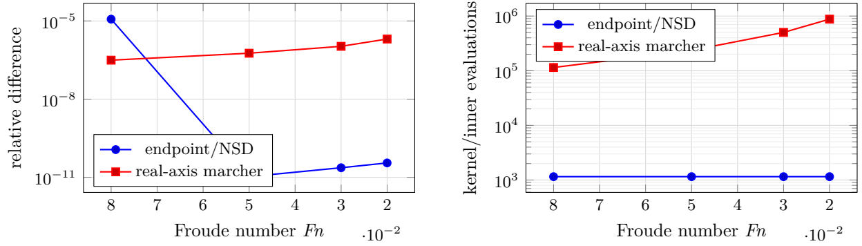
Figure 1: Observed accuracy (left) and work (right) as Froude number decreases. The endpoint/NSD accuracy below Fn = 0.05 is limited by the independent reference, while its quadrature work is fixed by geometry.
