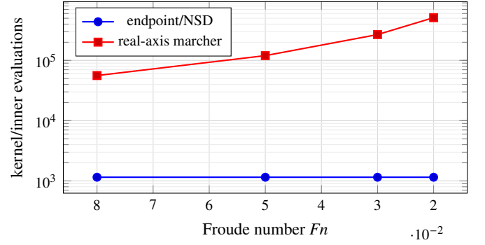
Figure 1: Observed accuracy (left) and work (right) as Froude number decreases. The deepened independent reference resolves endpoint/NSD differences down to the 10^{-13} – 10^{-12} level, while its quadrature work is fixed by geometry. At default tolerance the hybrid rejects the reduced result at F_n = 0.08 and accepts it at F_n = 0.05, 0.03, 0.02 .
