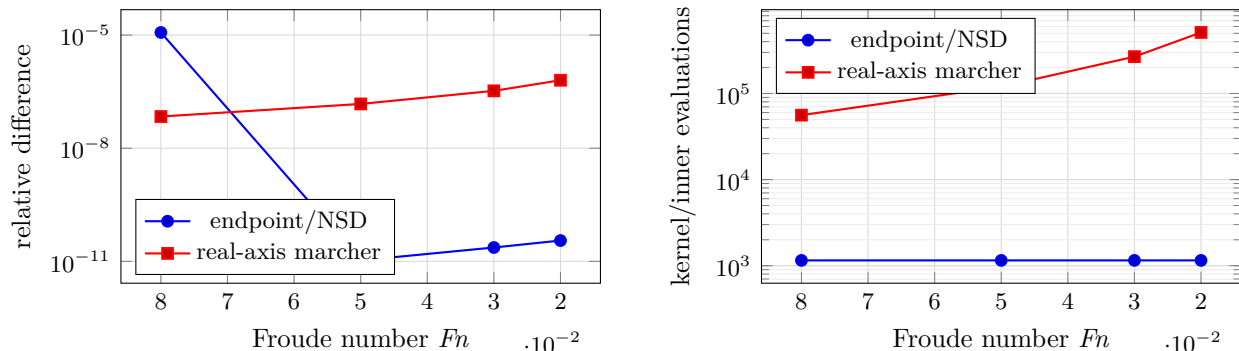
Figure 1: Observed accuracy (left) and work (right) as Froude number decreases. The endpoint/NSD accuracy below F_n = 0.05 is limited by the independent reference, while its quadrature work is fixed by geometry.
