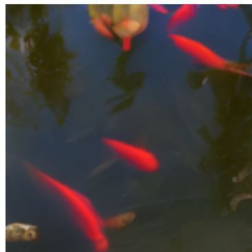
Ours ( N = 4 )
