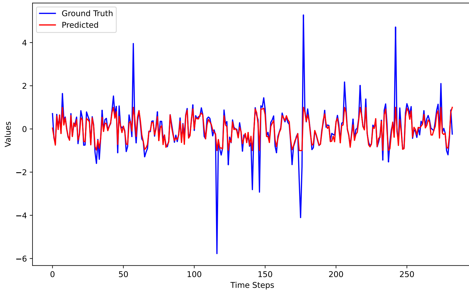
T - Nonsentiment: Ground Truth vs Predicted
