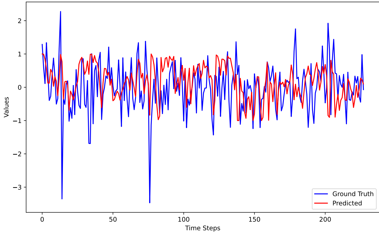
DIS - Nonsentiment: Ground Truth vs Predicted
