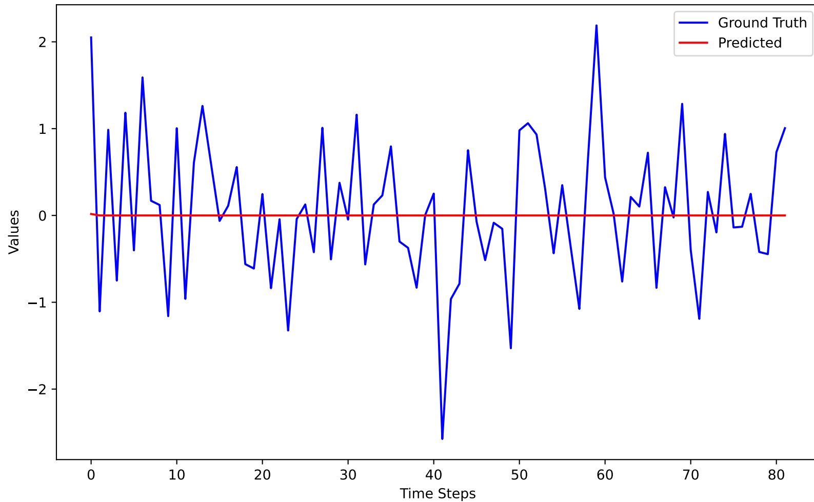
TSLA - Sentiment: Ground Truth vs Predicted
