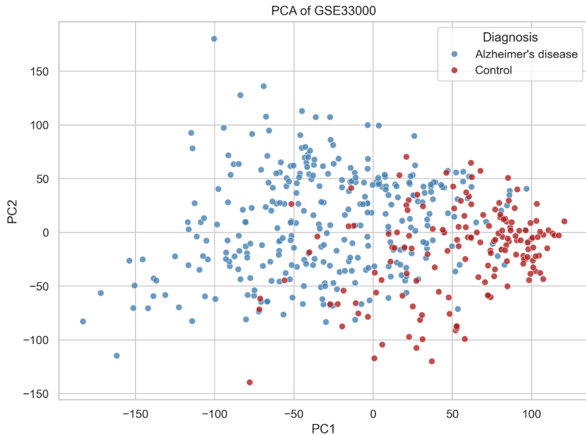
Figure 4. Principal Component Analysis (PCA) of GSE33000 samples.
