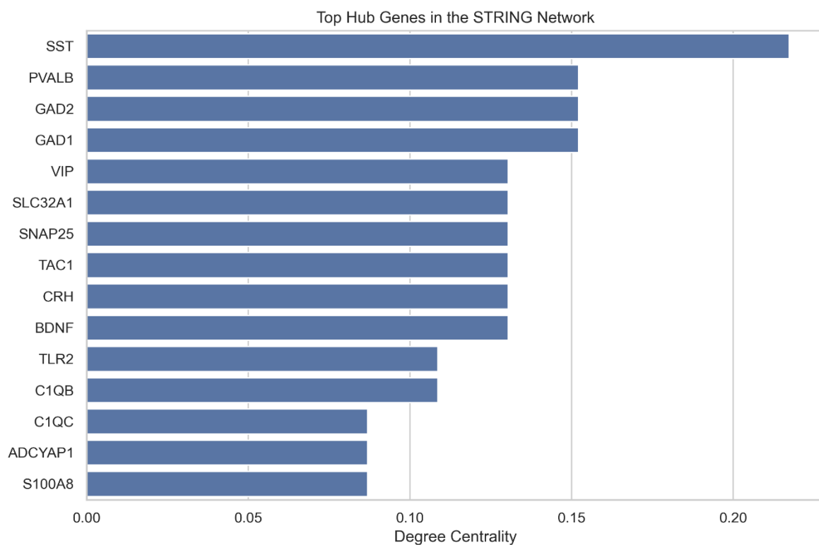
Figure 11. Hub genes ranked according to degree centrality within the protein–protein interaction network.
