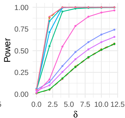
Model 3.ii.
