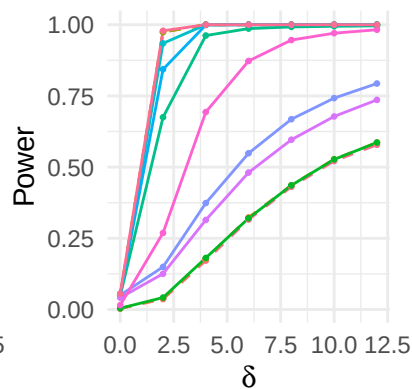
Model 3.iii.
