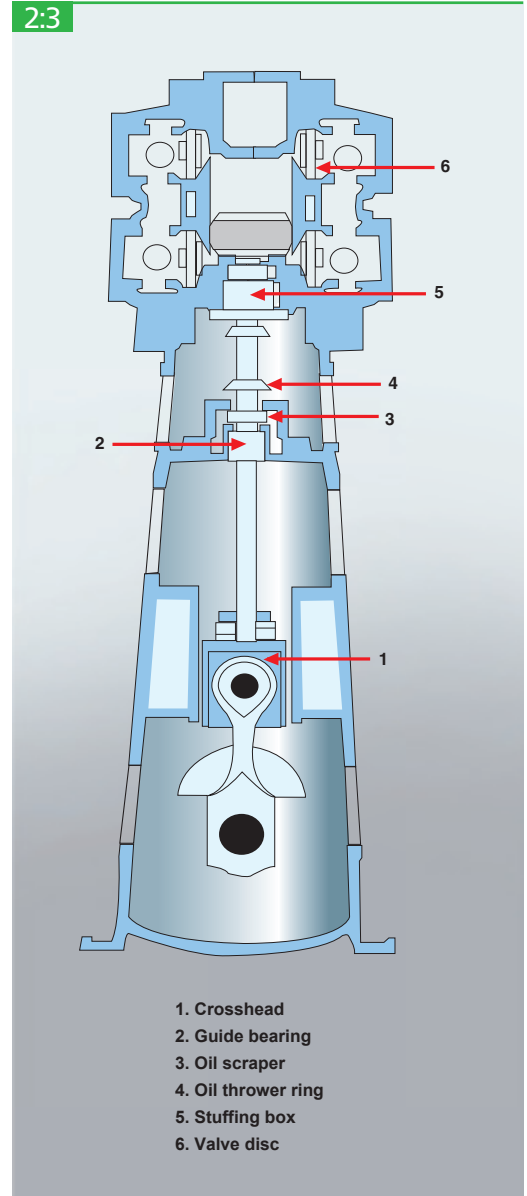
Labyrinth sealed, double acting oil-free piston compressor with crosshead.
