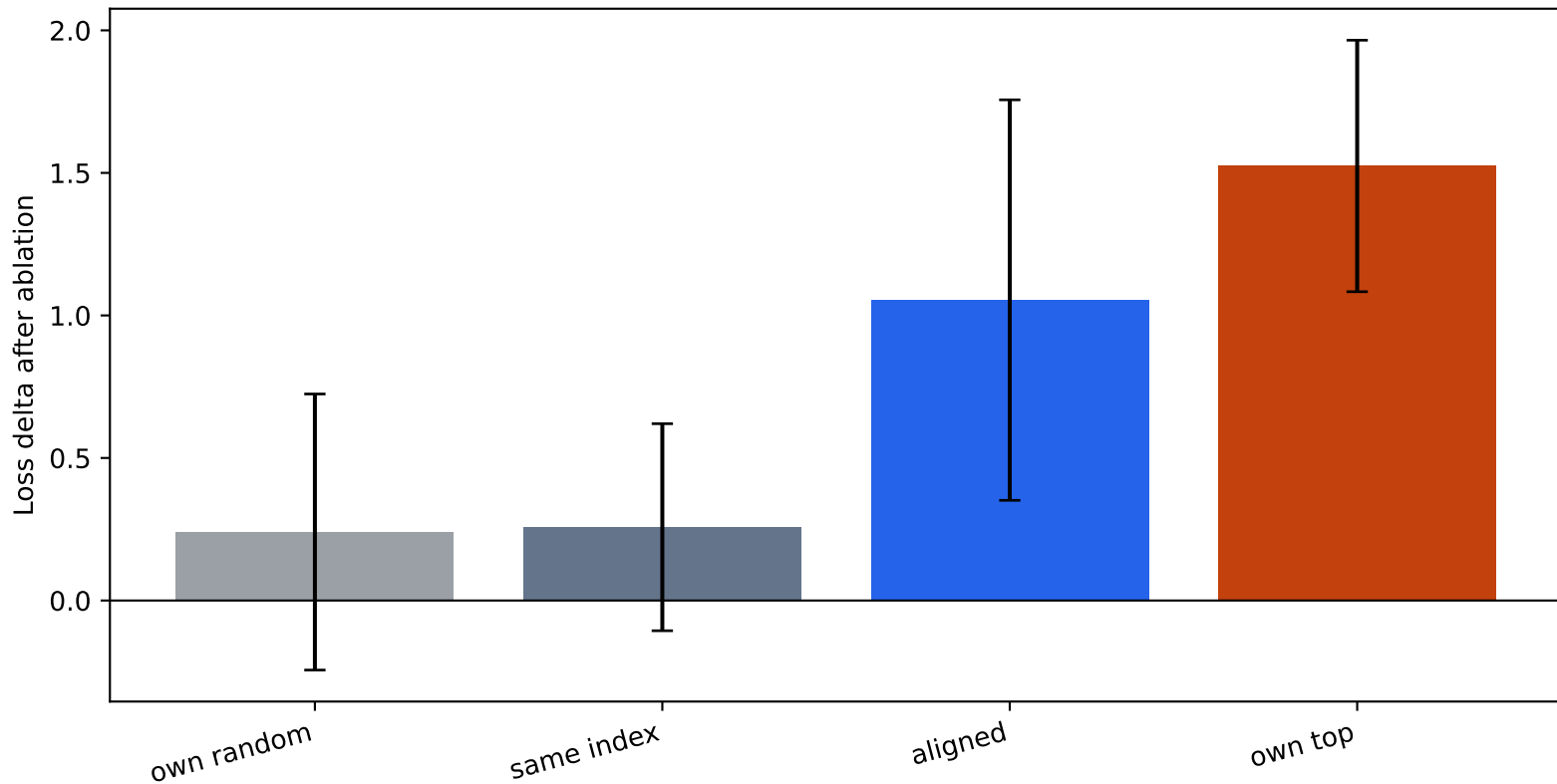
Top repeat-match heads are causally important
