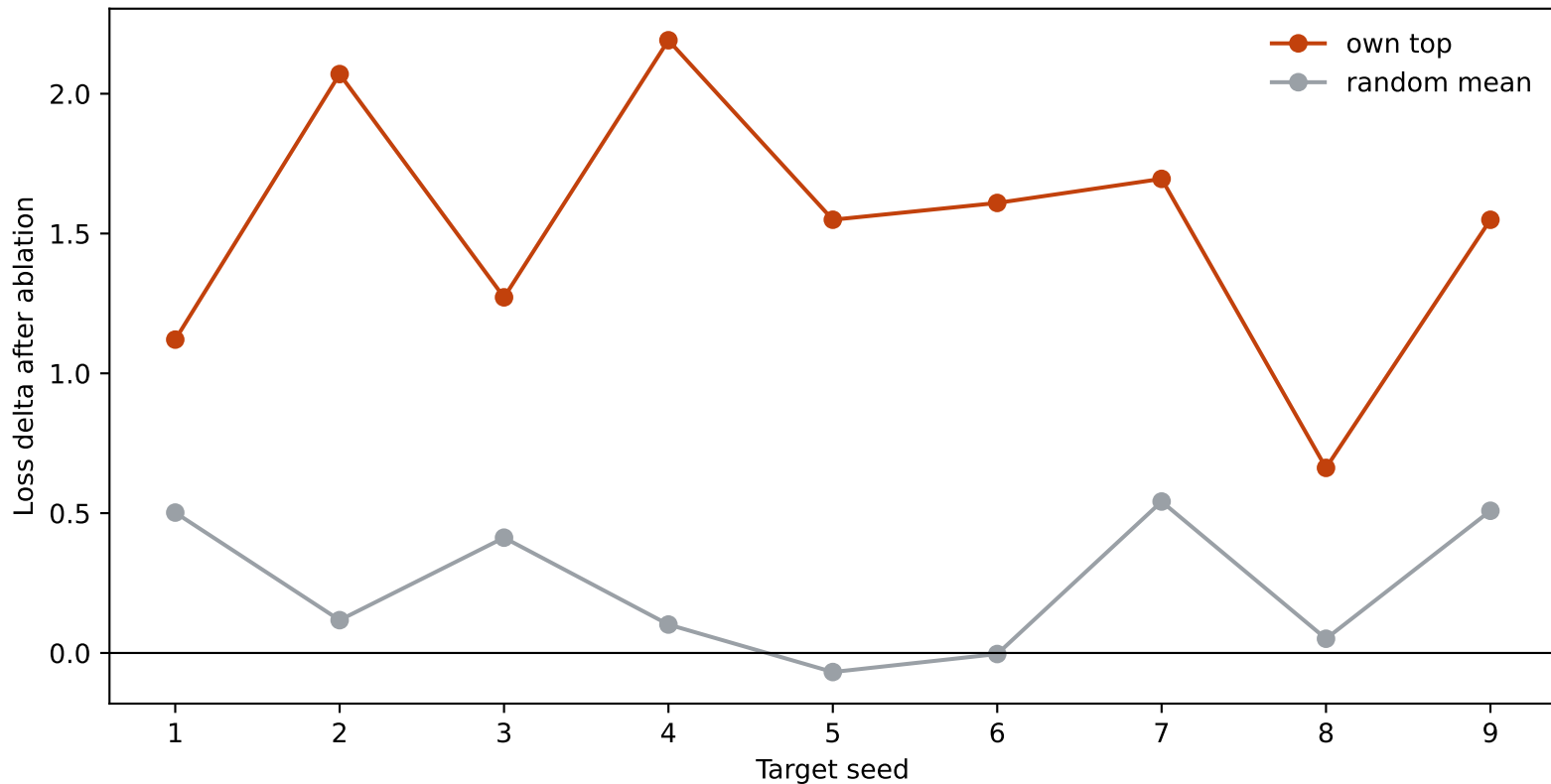
Own top heads beat random controls in every seed
