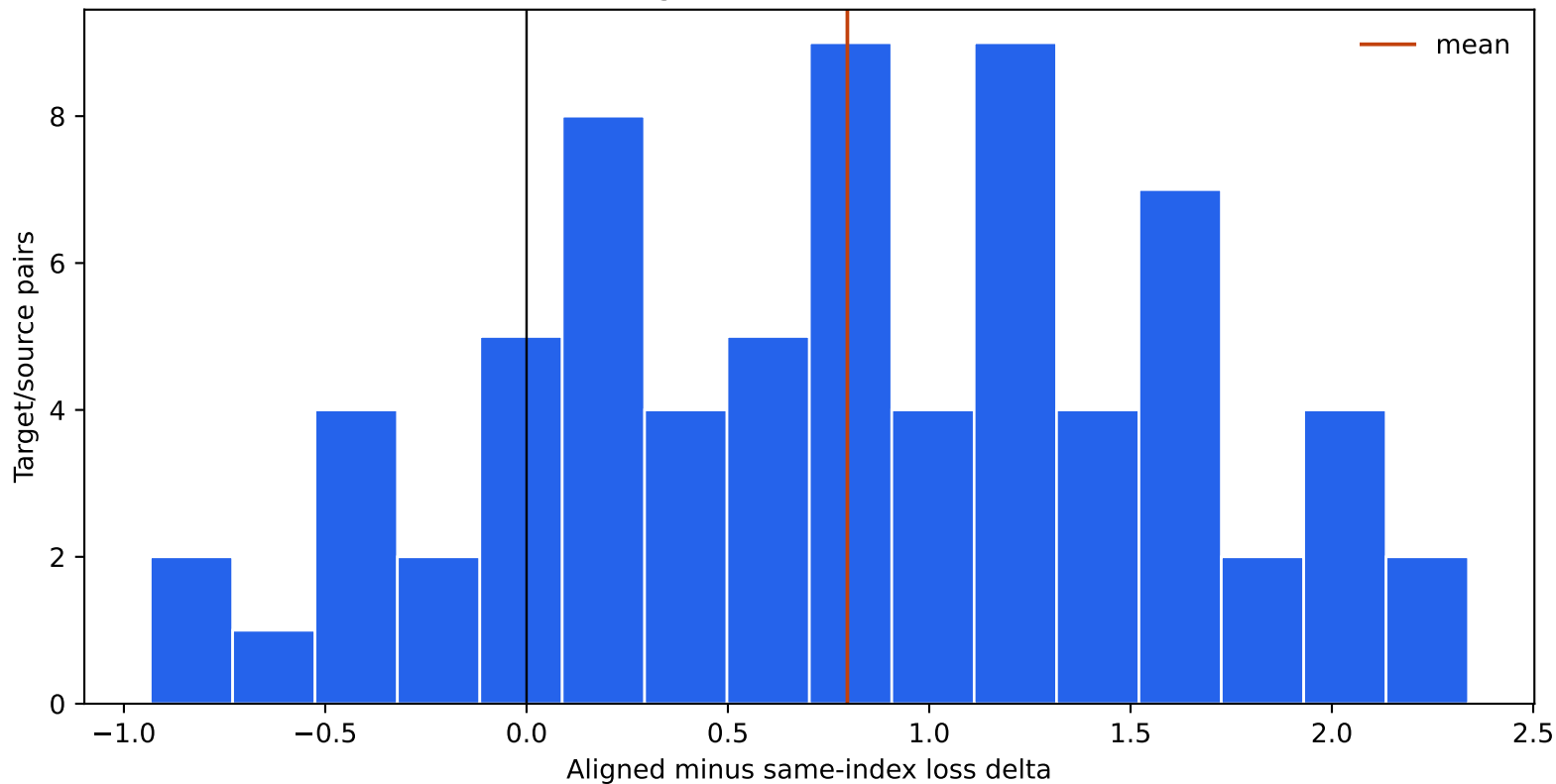
Raw-score alignment transfers the causal role
