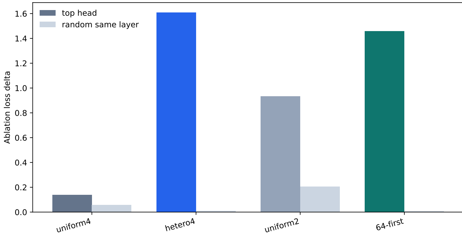
The heterogeneous 64-dim slot is causally load-bearing
