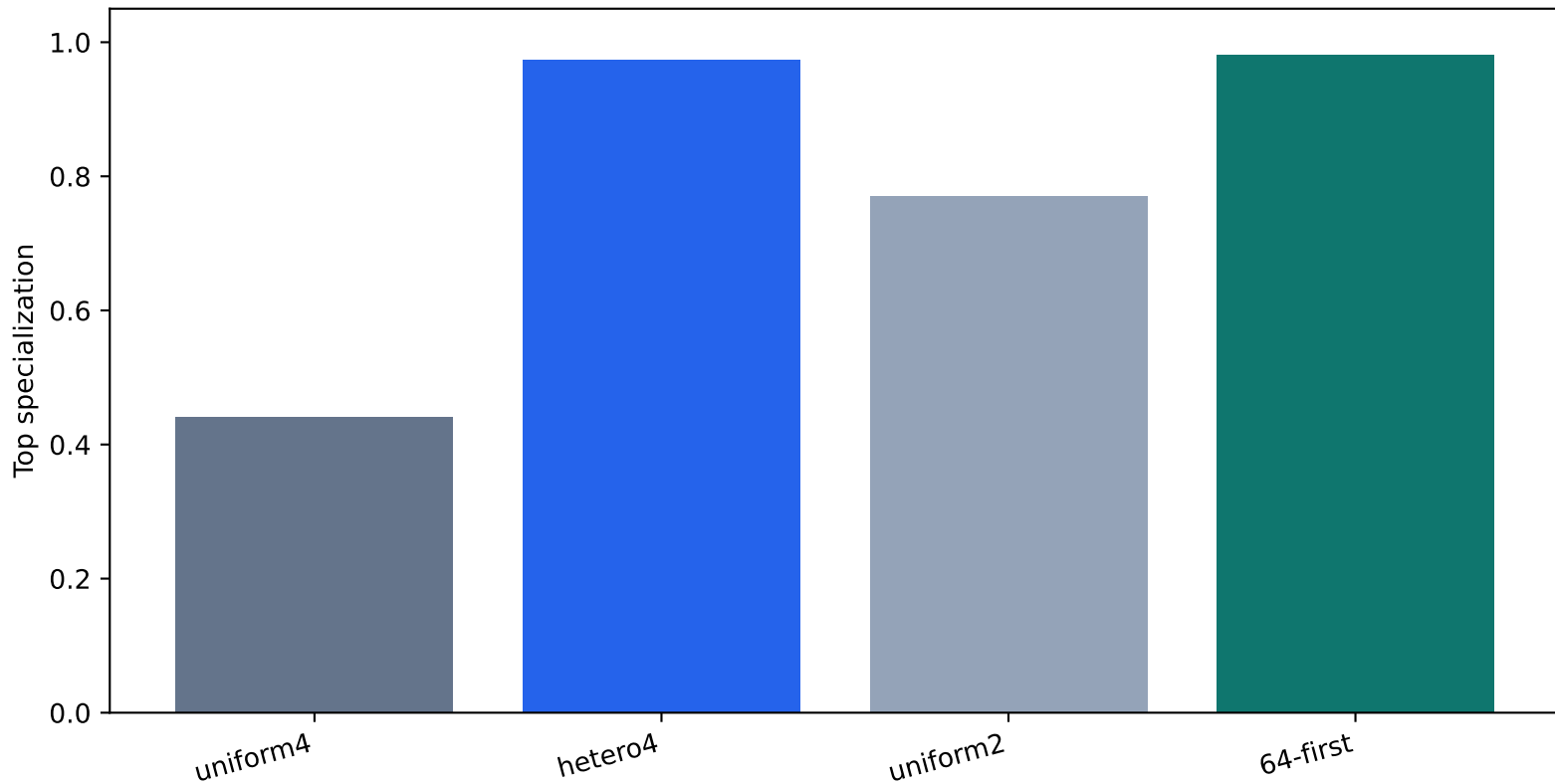
Heterogeneous head dimensions concentrate causal specialization
