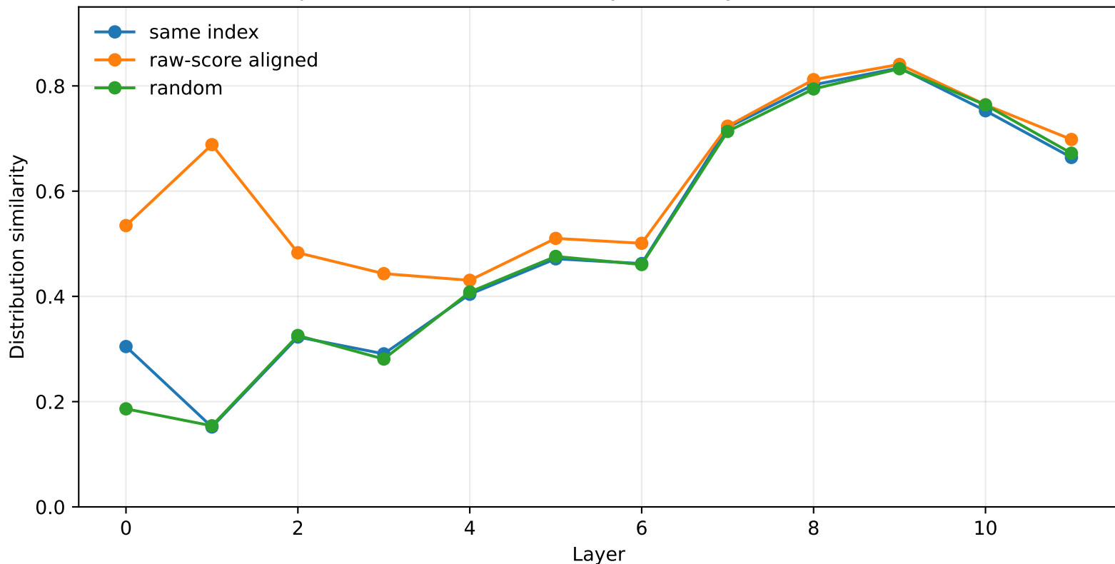
Repeat-match role consistency across Pythia-160M seeds
