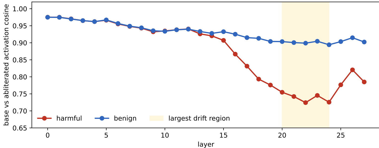
Prompt-selective activation drift
