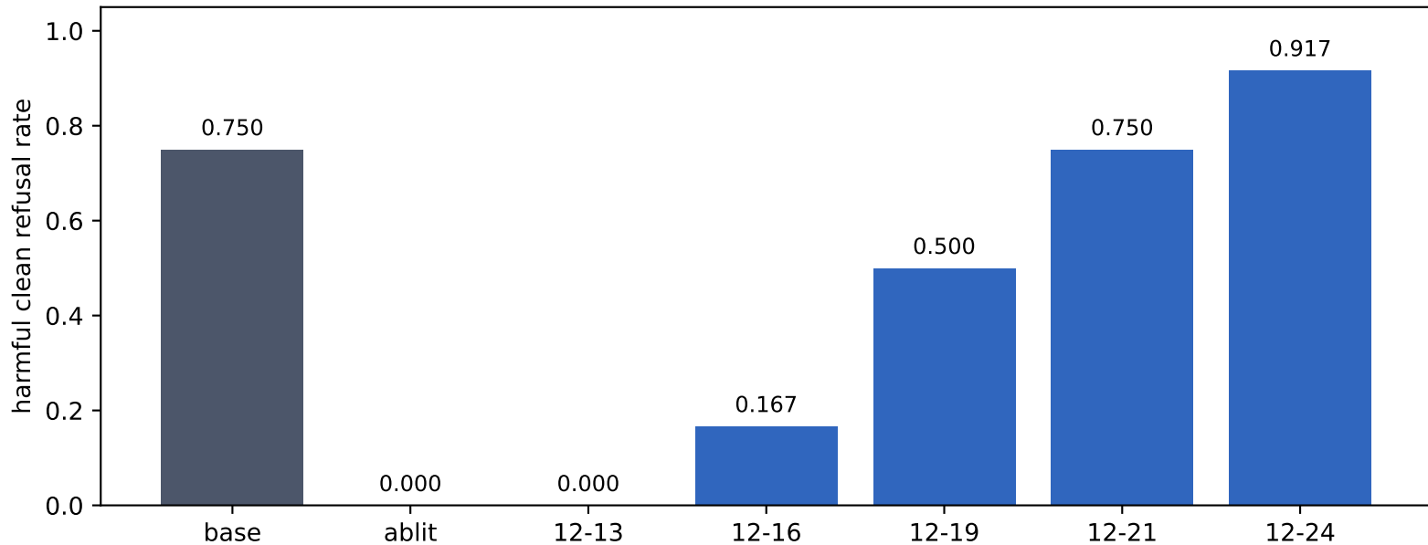
Static MLP patch localization: broad range needed
