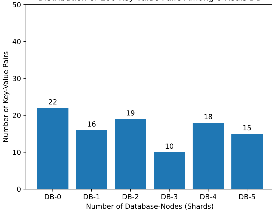
Distribution of 100 Key-Value Pairs Among 6 Redis DB
