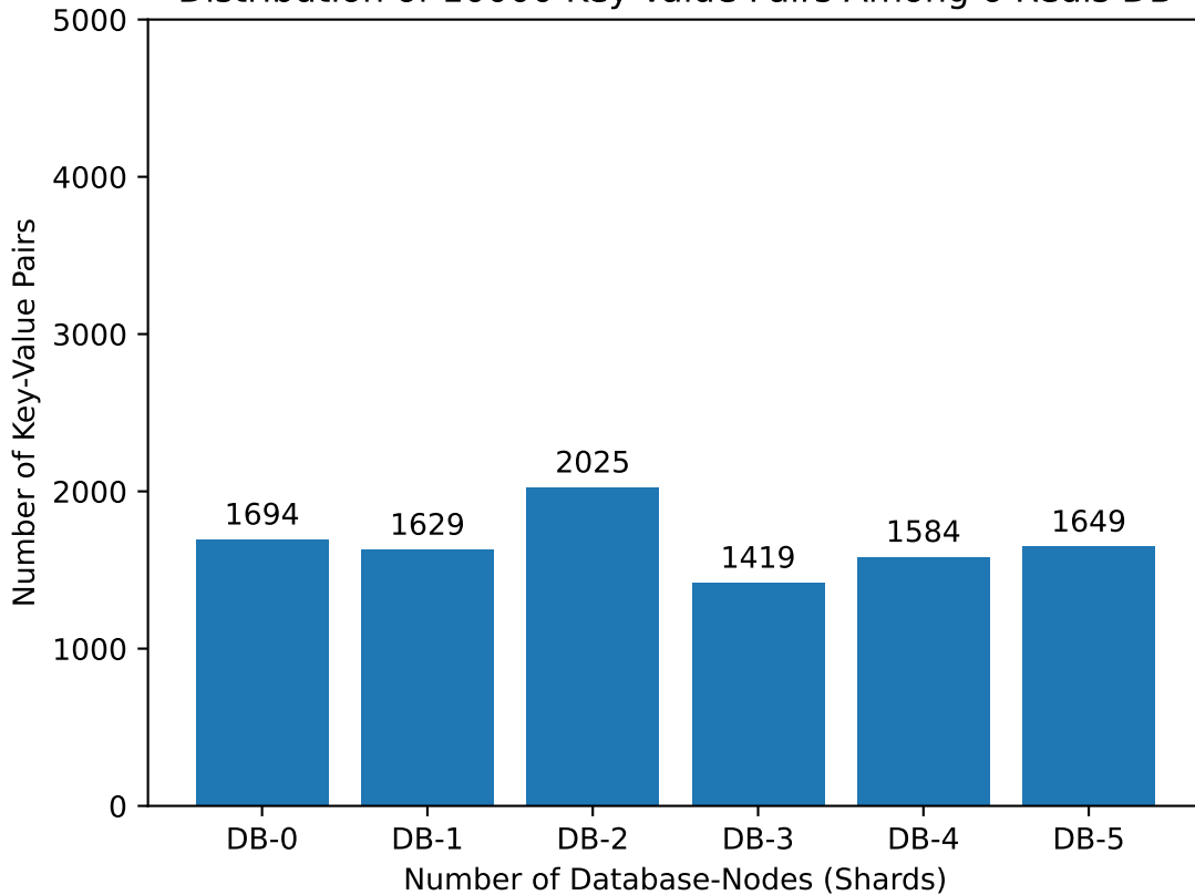
Distribution of 10000 Key-Value Pairs Among 6 Redis DB
