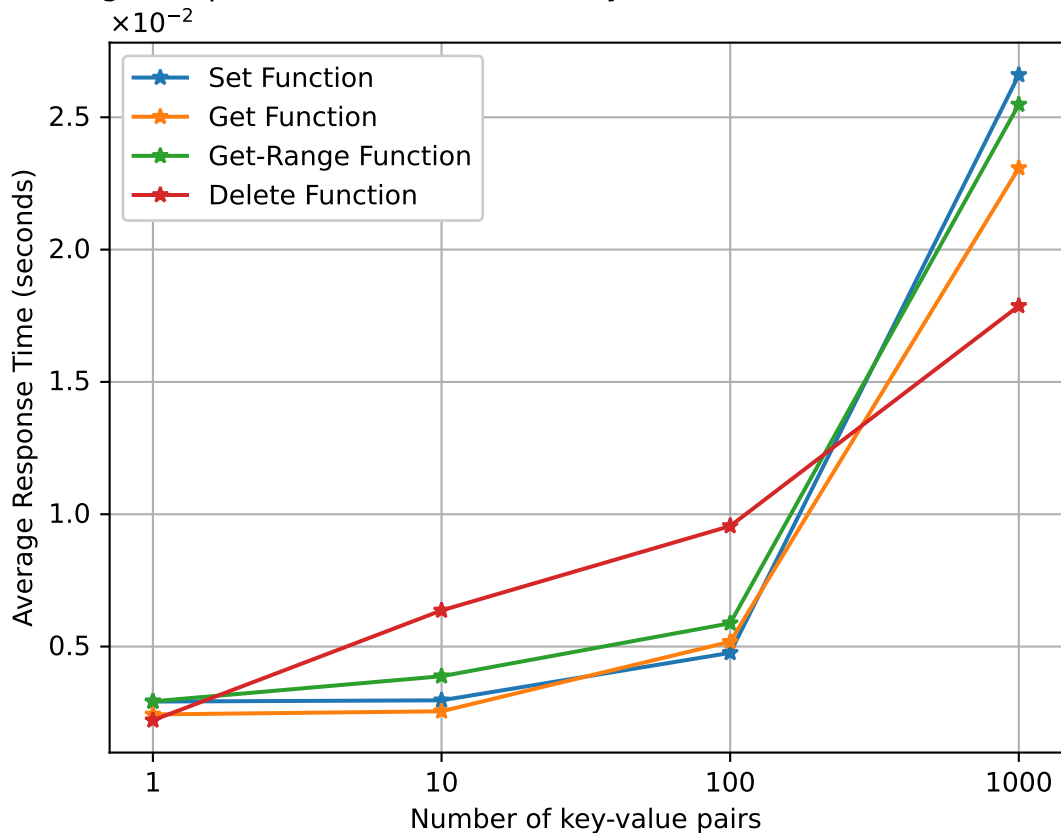
Average Response Time Per Given Key-Value Pairs (Without Middleware)
