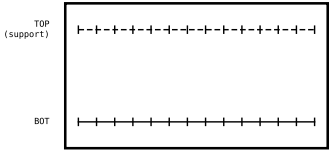
3. SLAB SECTION (5"-6" THICK, TWO-WAY)
