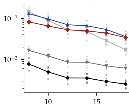
random 3-regular
