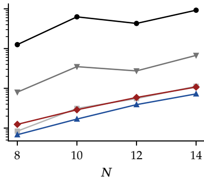
random 3-regular
