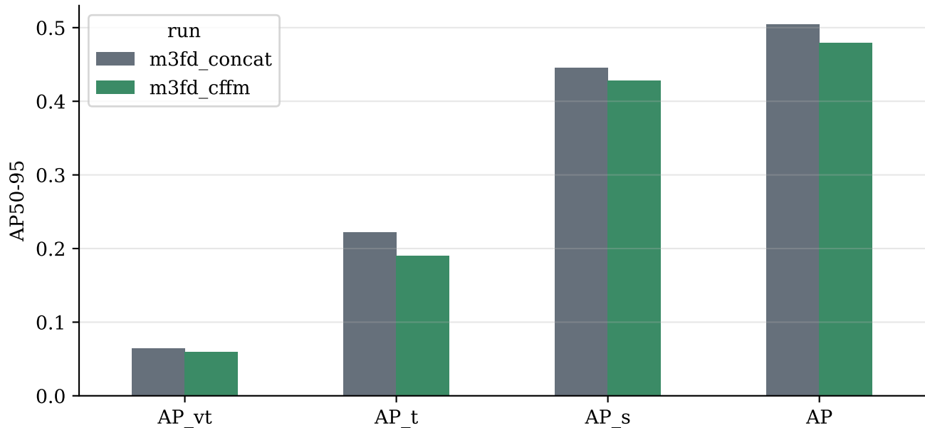
M3FD by object size
