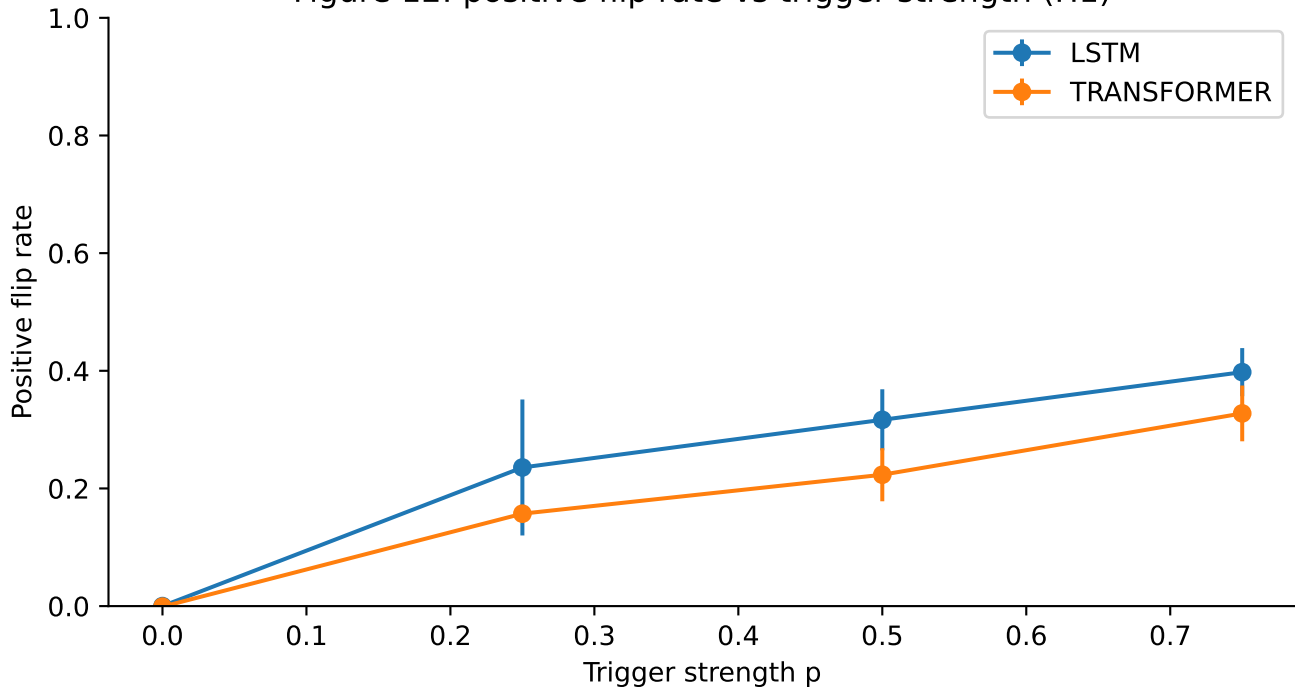
Figure 12: positive flip rate vs trigger strength (H1)
