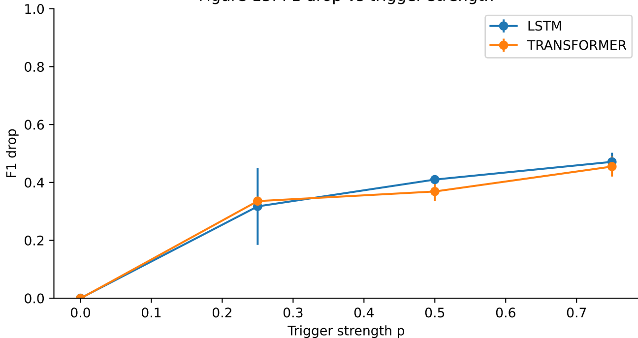
Figure 13: F1 drop vs trigger strength
