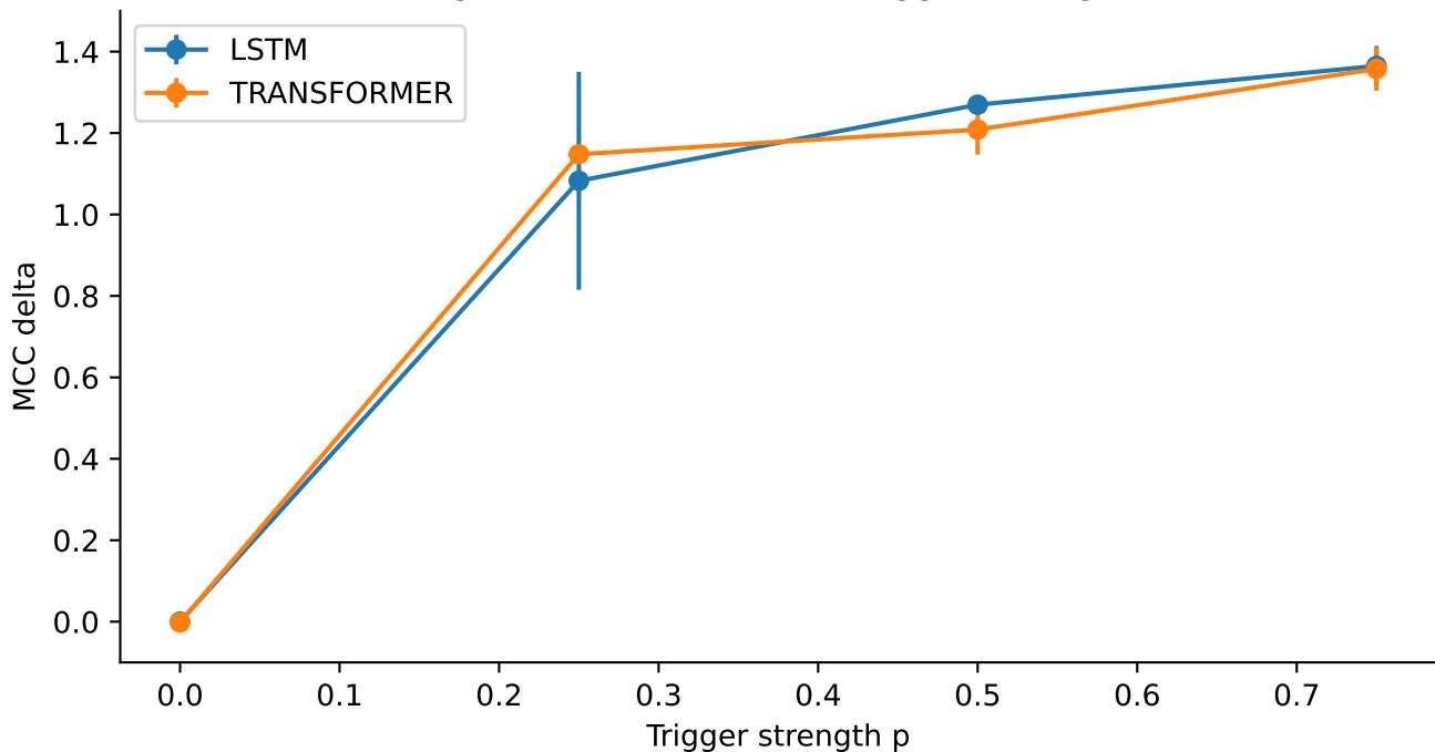
Figure 14: MCC delta vs trigger strength
