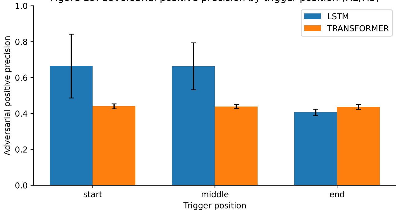
Figure 19: adversarial positive precision by trigger position (H2/H3)
