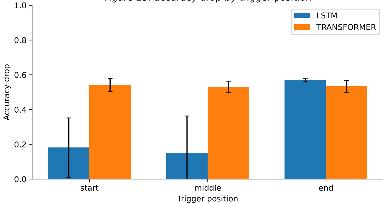
Figure 23: accuracy drop by trigger position
