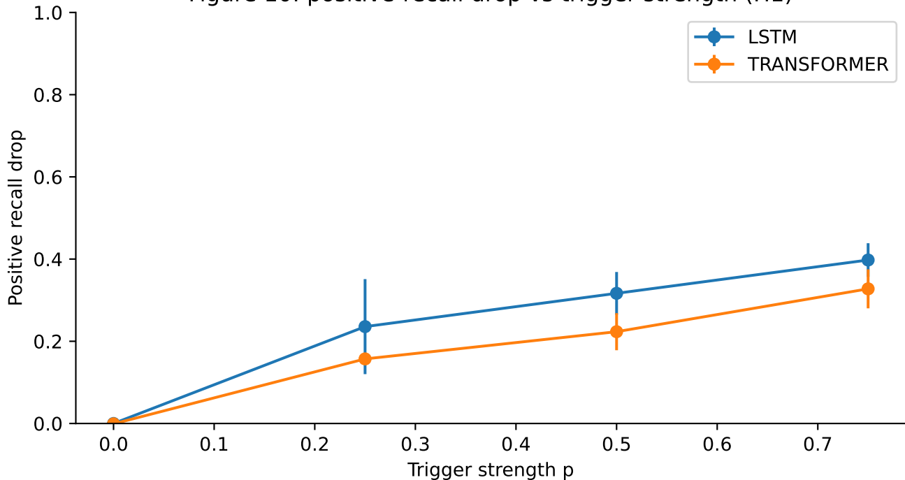
Figure 10: positive-recall drop vs trigger strength (H1)
