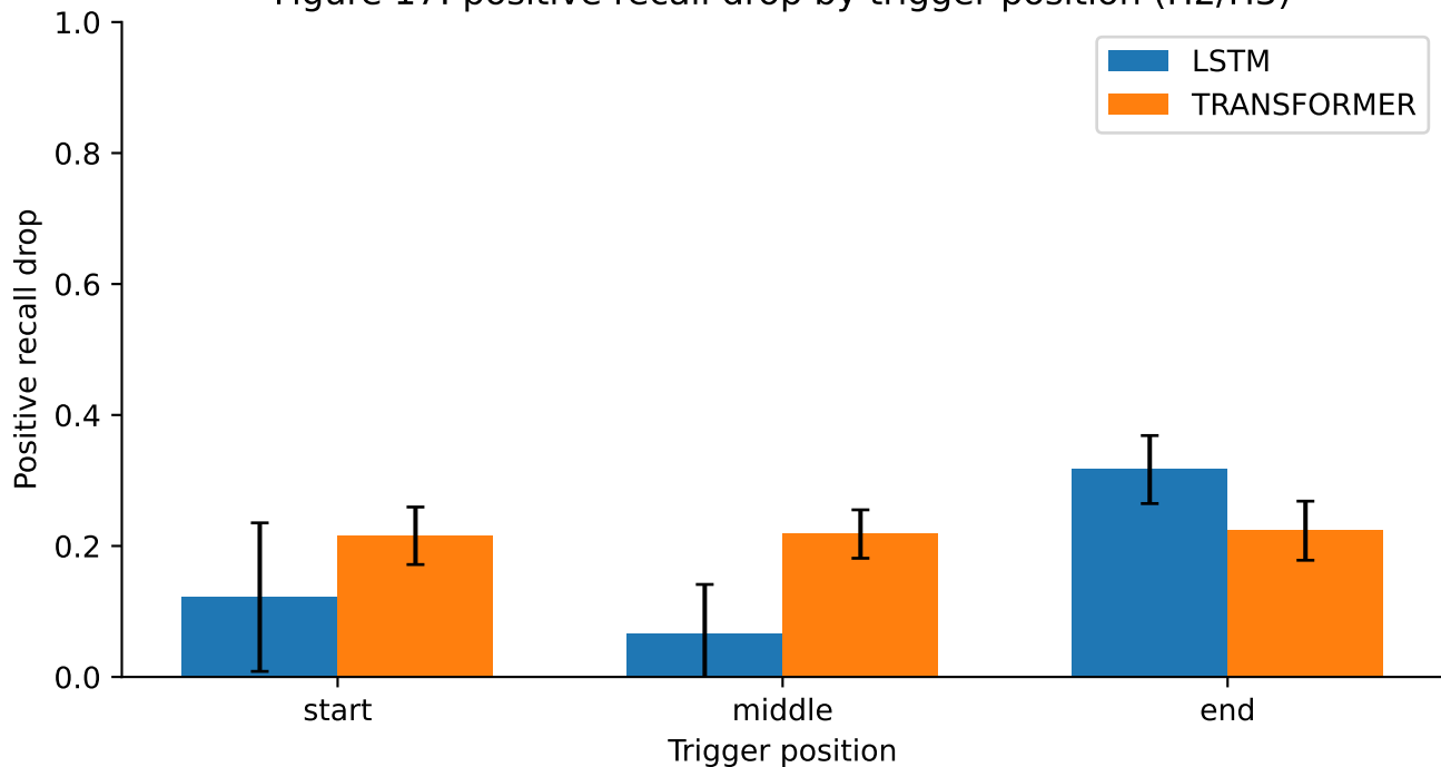
Figure 17: positive recall drop by trigger position (H2/H3)
