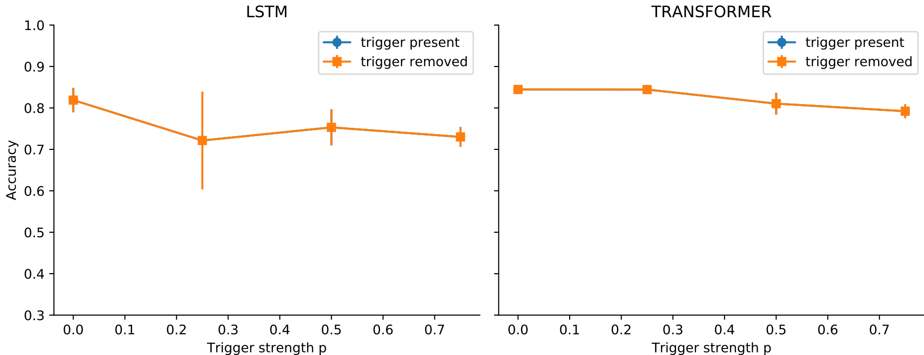
Figure 1: shortcut reliance on positive class (H1)
