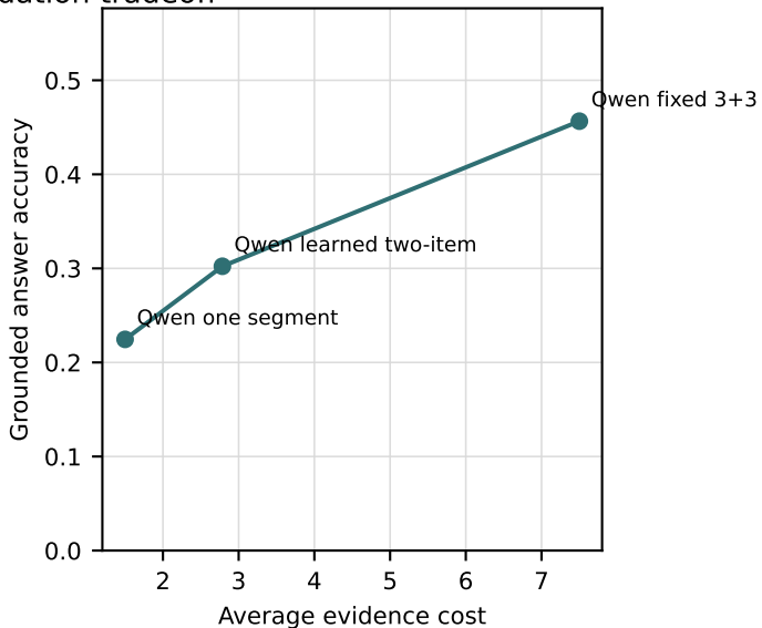
NEXT-GQA validation tradeoff
