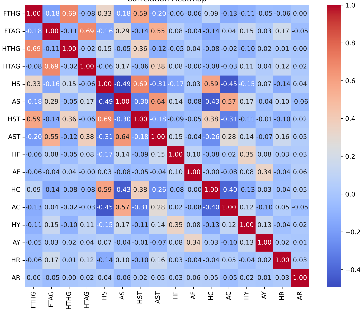
Correlation Heatmap
