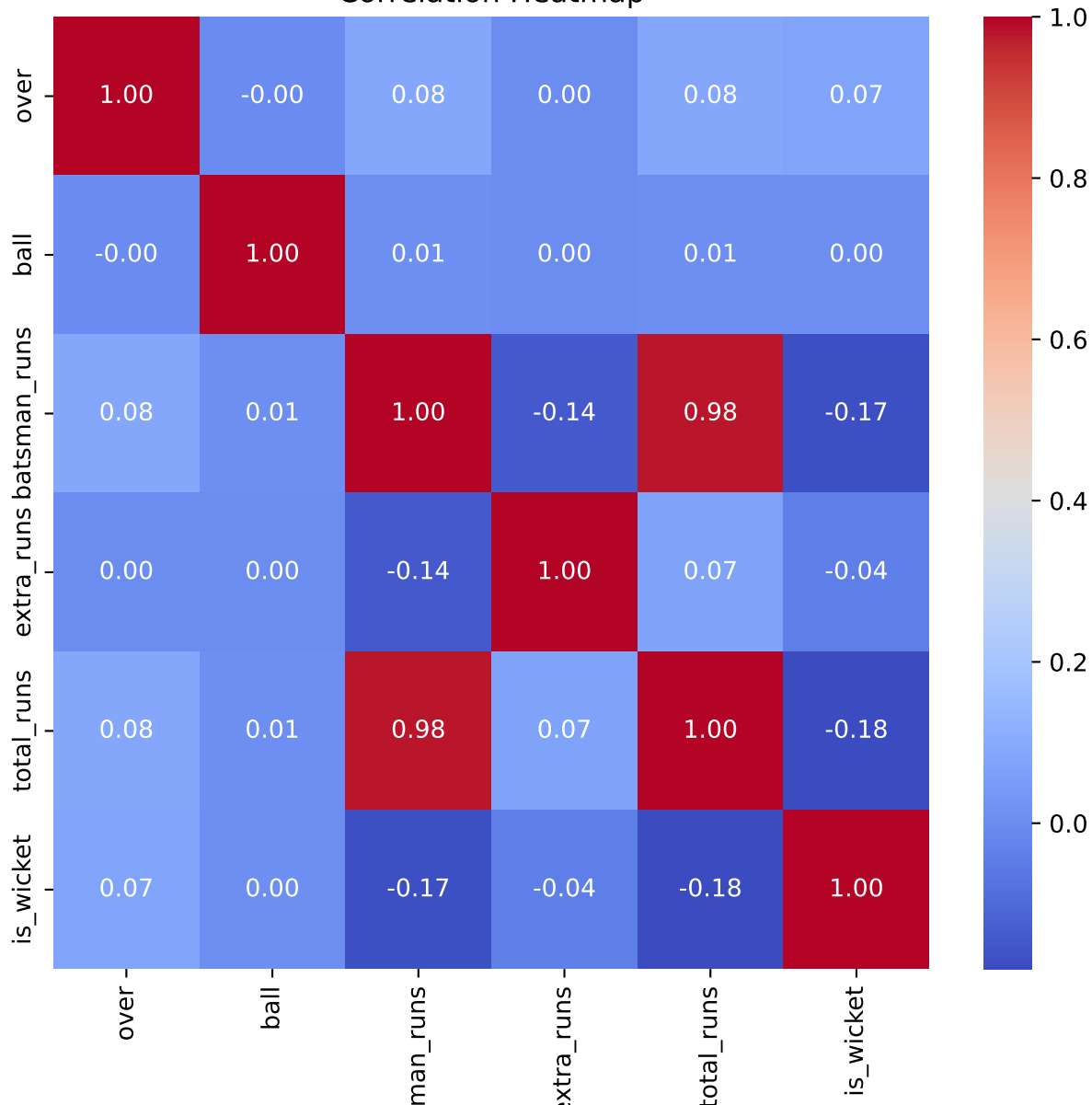
Correlation Heatmap
