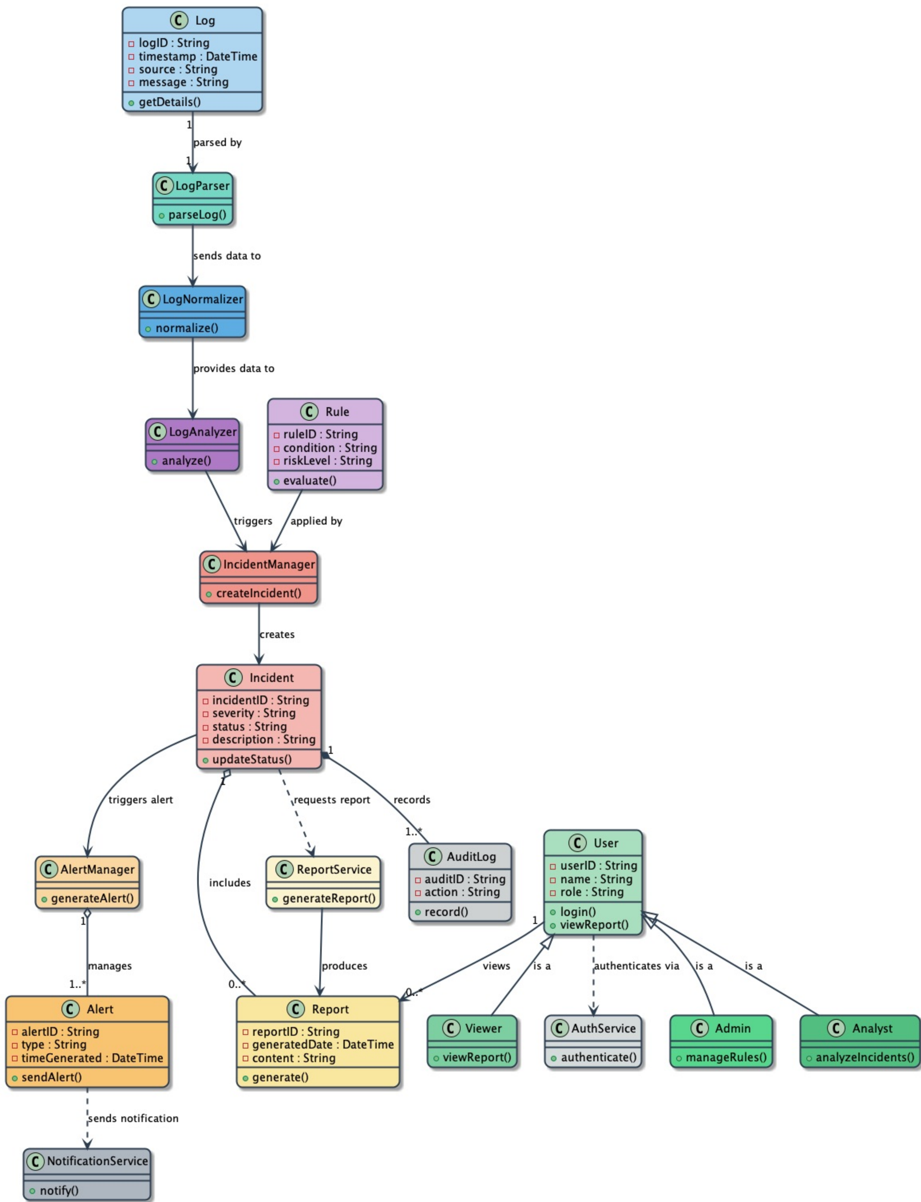
ALARS — CLASS DIAGRAM
