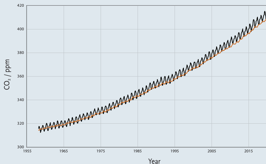
FIGURE B2. Measurements of atmospheric CO 2 since 1958 from the Mauna Loa Observatory in Hawaii (black) and from the South Pole (red) show a steady annual increase in atmospheric CO 2 concentration. The measurements are made at remote places like these because they are not greatly influenced by local processes, so therefore they are representative of the background atmosphere. The small up-and-down saw-tooth pattern reflects seasonal changes in the release and uptake of CO 2 by plants. Source: Scripps CO 2 Program
