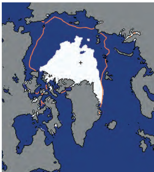
FIGURE 5. The Arctic summer sea ice extent in 2012, (measured in September) was a record low, shown (in white) compared to the median summer sea ice extent for 1979 to 2000 (in orange outline). In 2013, Arctic summer sea ice extent rebounded somewhat, but was still the sixth smallest extent on record. In 2019, sea ice extent effectively tied for the second lowest minimum in the satellite record, along with 2007 and 2016—behind only 2012, which is still the record minimum. The 13 lowest ice extents in the satellite era have all occurred in the last 13 years. Source: National Snow and Ice Data Center
