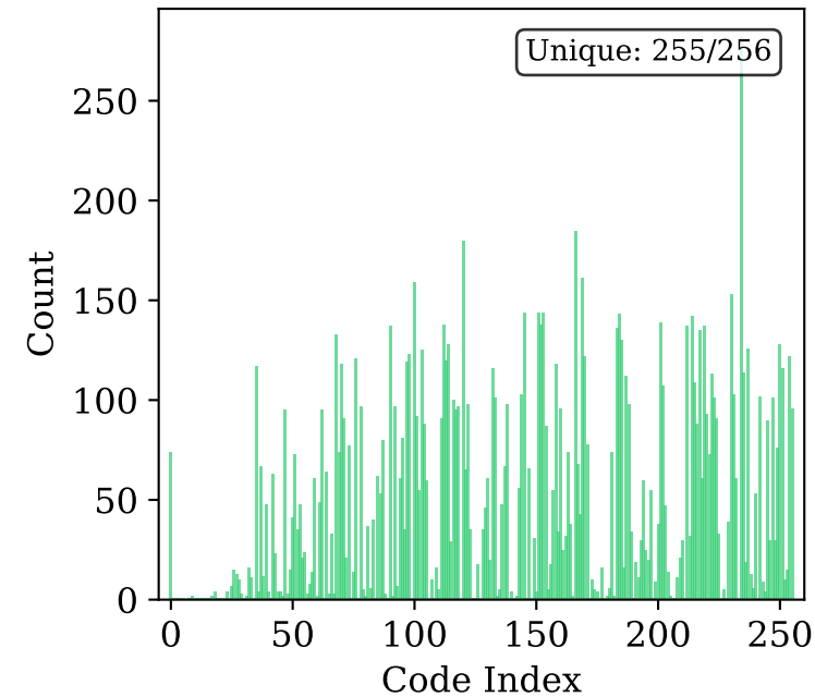
CSJ-ID Level 3
