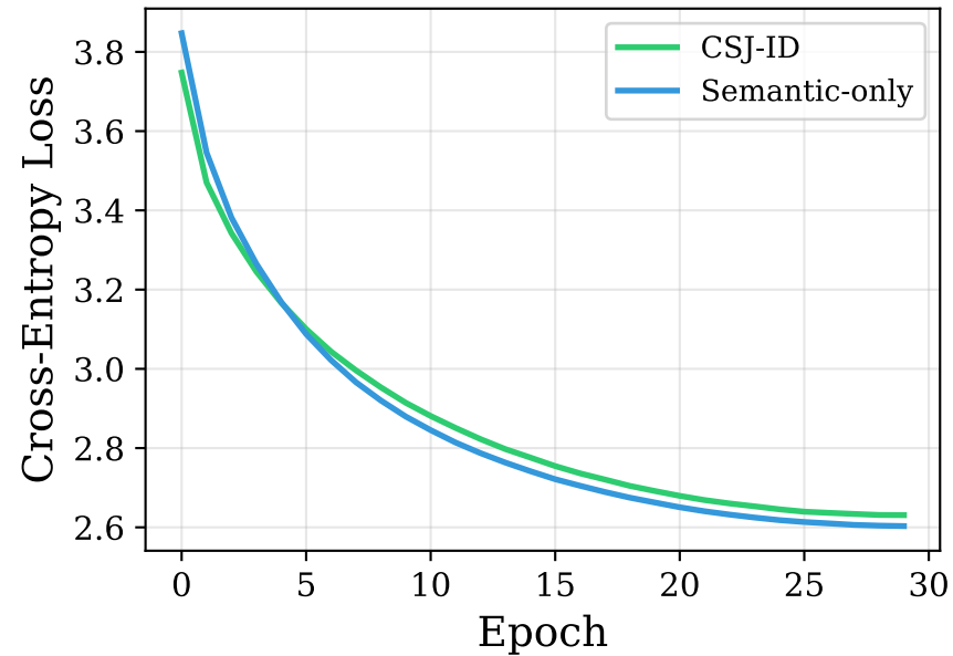
GenRec Training
