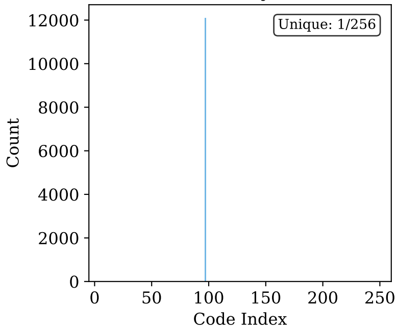
Semantic-only Level 1
