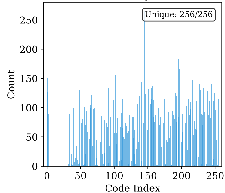
Semantic-only Level 4
