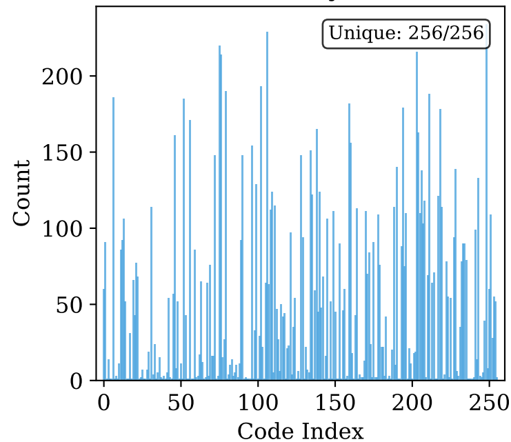
Semantic-only Level 2
