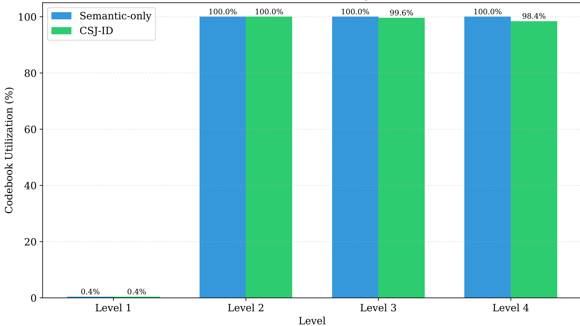
Codebook Utilization by Level
