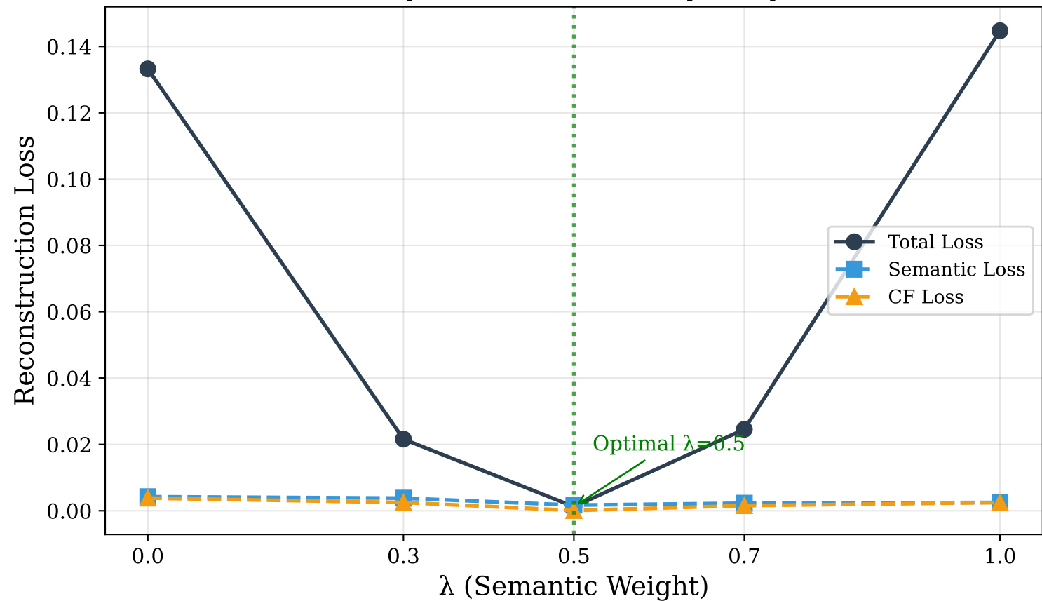
Beauty - Lambda Sensitivity Analysis
