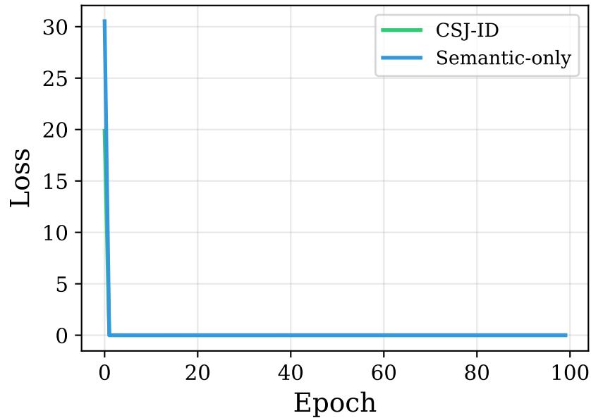
RQ-VAE Training
