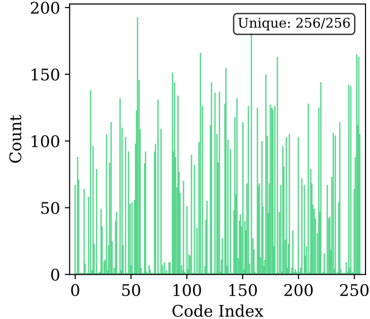
CSJ-ID Level 2
