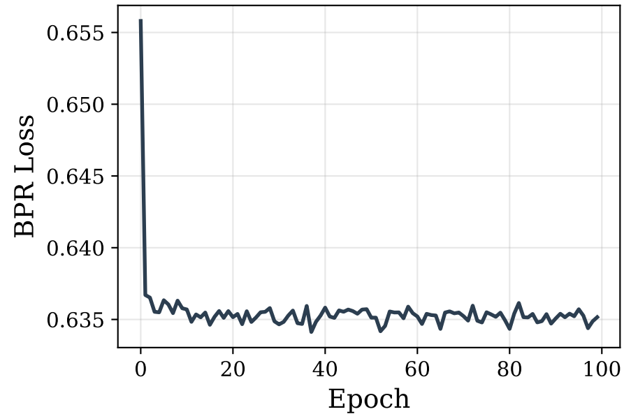
LightGCN Training
