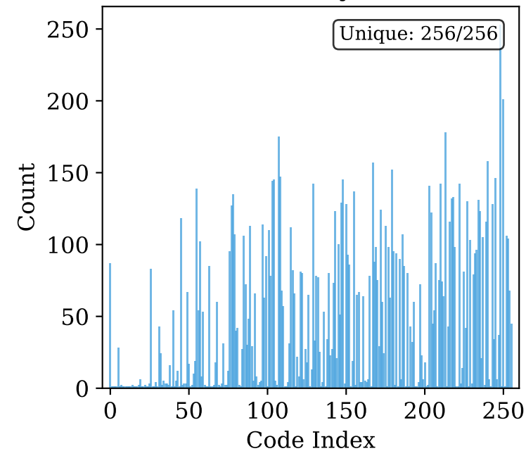
Semantic-only Level 3
