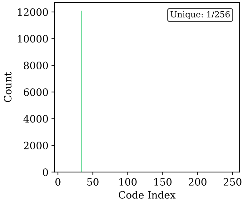
CSJ-ID Level 1
