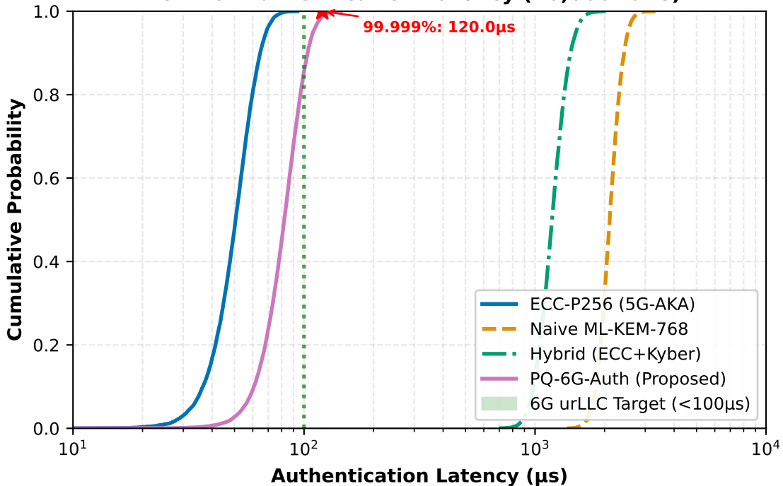
CDF of Authentication Latency (10,000 runs)
