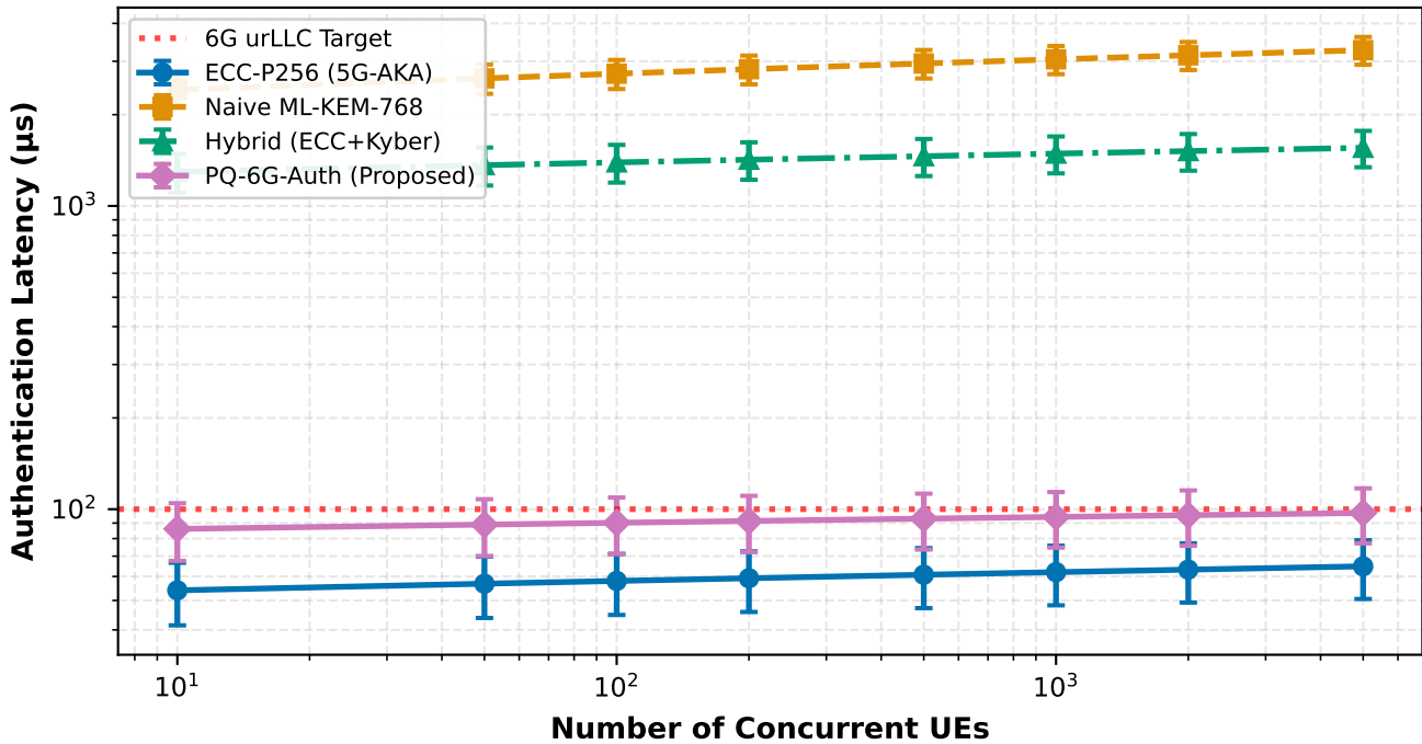
Scalability: Latency vs. Number of UEs
