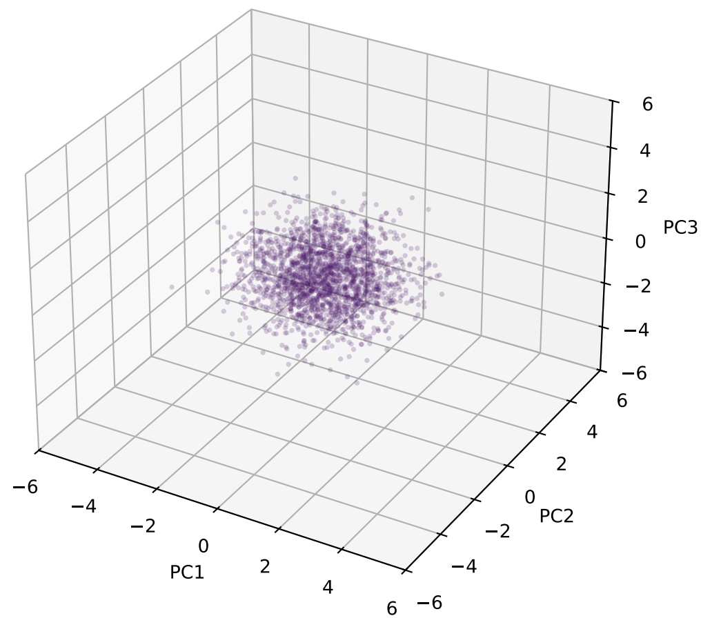
shuffled pairs
