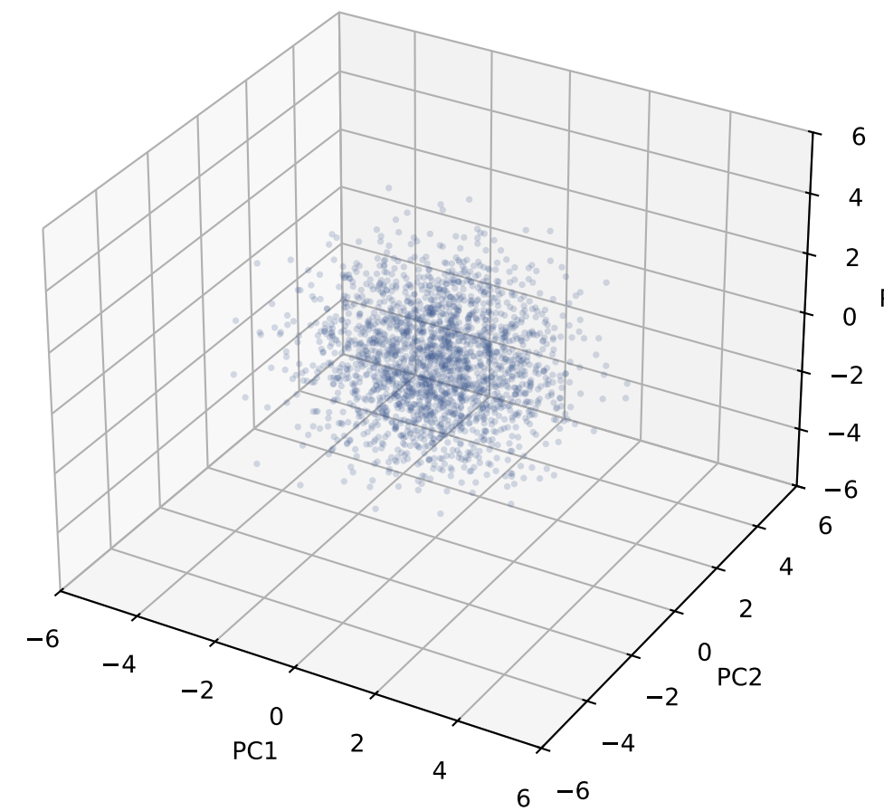
uniform actions
