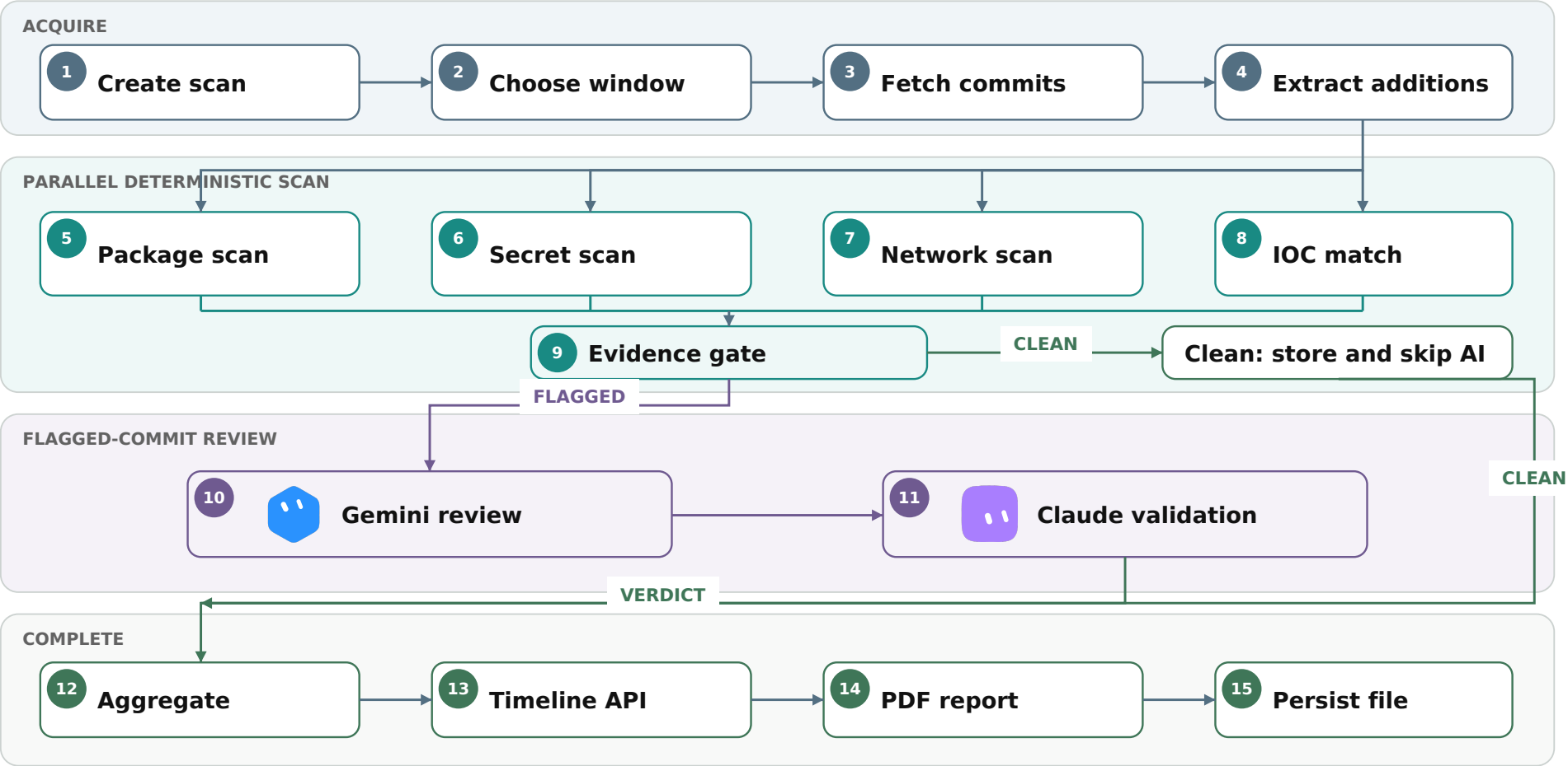
Figure 2: Per-commit analysis and conditional consensus lifecycle.
