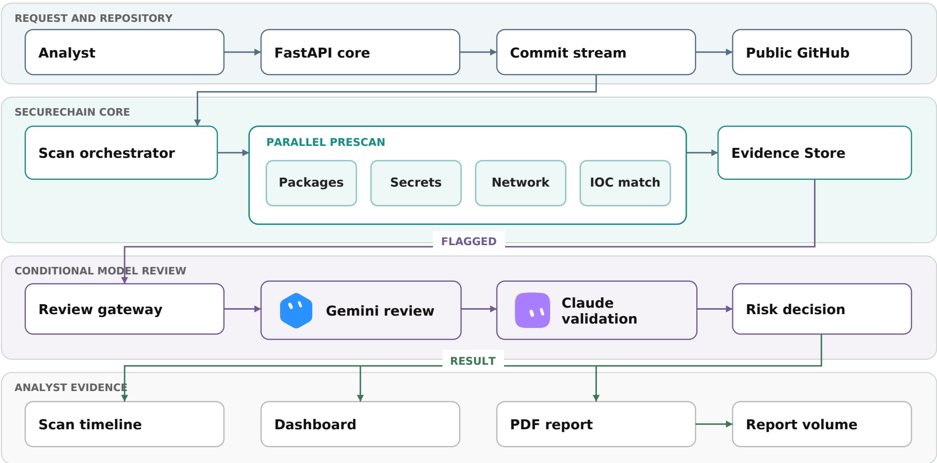
Figure 1: SecureChain logical architecture and trust boundaries.
