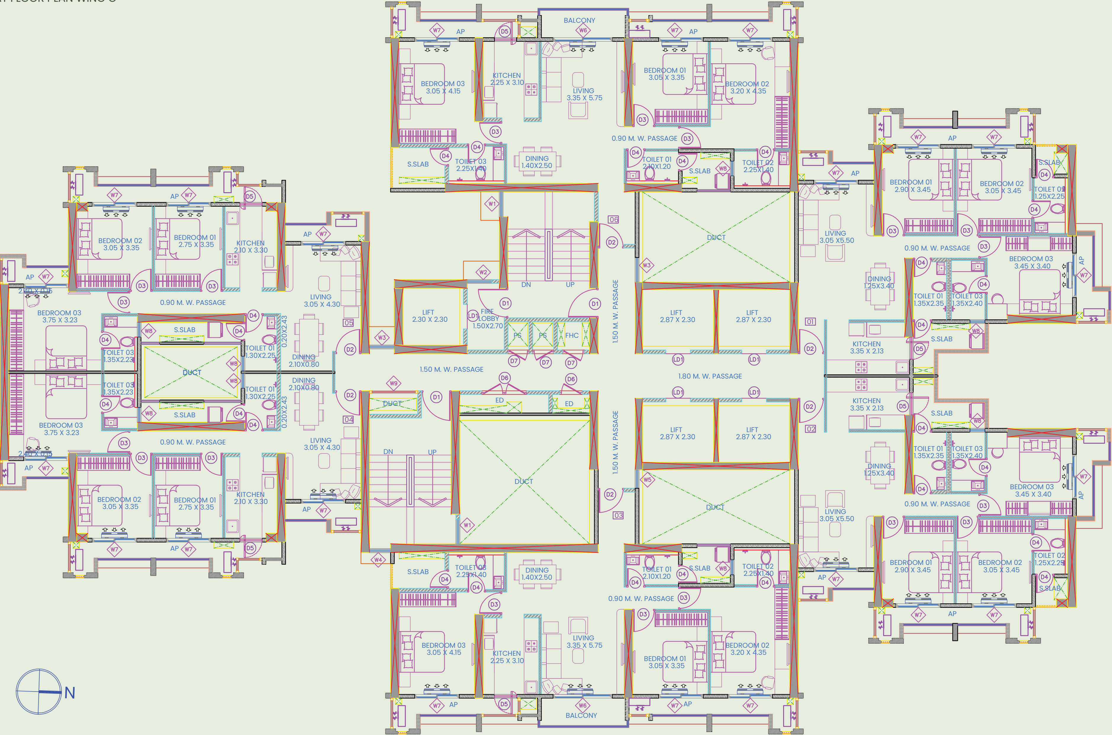
FLAT FLOOR PLAN WING G
