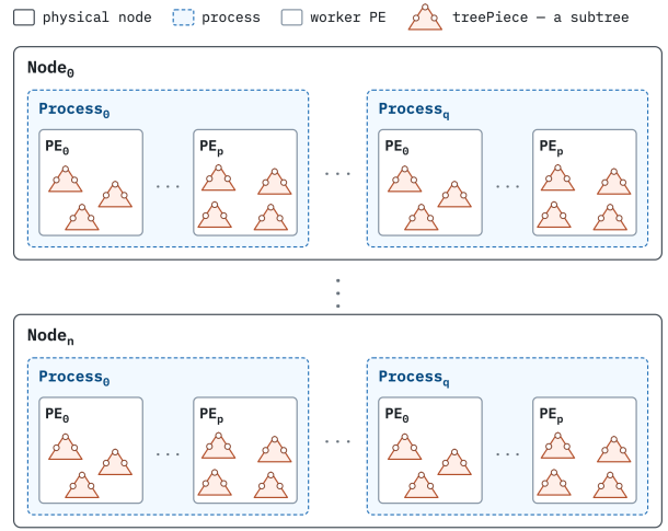
Fig. 1. Machine Hierarchy with Nodes, Processes, PEs, and TreePiece Chares
