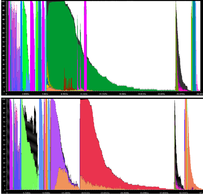
Fig. 2. Time profiles of the code before ParaTreeT2 on 120 cores; white is idle, black system overhead. Top: triggered stop-everything phases (pink) compressing process-local paths, inside the tree traversal (green). Bottom: two traversals; the first spike and fall is the local-only traversal, the second the remote one. The phases separate cleanly, but the run is slower
