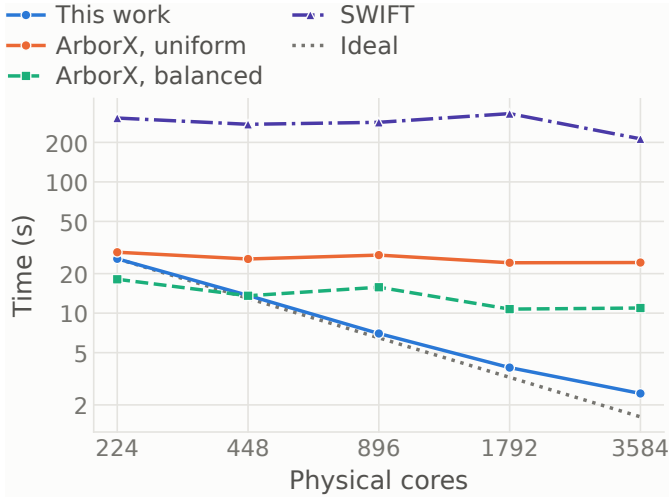
Fig. 10. Group-finding time on the 2B dataset on Frontier , 4 to 64 nodes at 56 physical cores per node, excluding decomposition and our tree build. ArborX is shown with an equal-volume and a count-balanced decomposition. Ideal scaling is anchored at our smallest run
