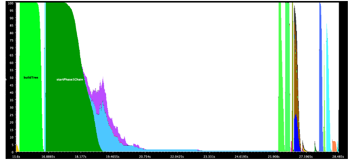
Fig. 8. Time profile of 16 node run (1792 cores) on Frontier , 2B particles 8 processes per node. Colors are as in Fig. 6: the sky-blue band with purple stacked on it is phase B, and the dark-blue band with brown stacked on it is the distributed walk
