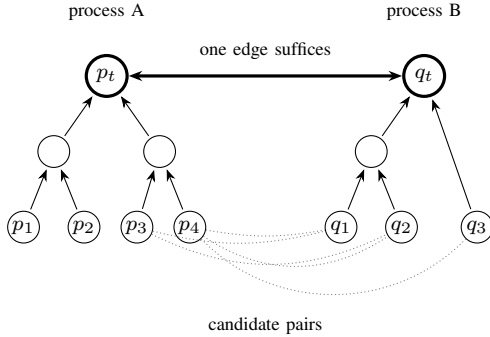
Fig. 3. Two inverted trees whose tips are on different processes. Every candidate pair found by the traversal (dotted) stands for the same edge between the tips (bold)
