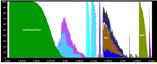
Fig. 6. Time profile of the entire cluster finding algorithm for 80 million particles on 480 cores. Some phases are labeled in the plot. Of the others, the sky-blue band with purple stacked on it is phase B, and the dark-blue band with brown stacked on it is the distributed walk
