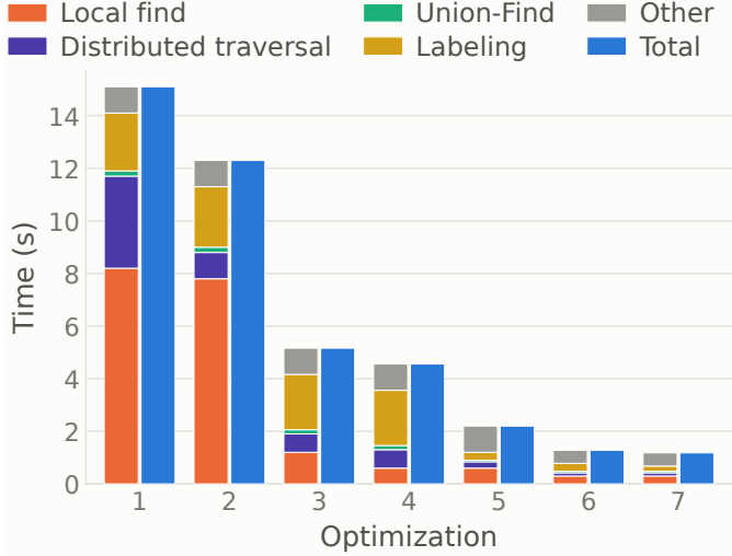
Fig. 7. Breakdown of how optimizations affect FoF on 80M dataset. Key phases (focuses of optimizations) are separated out. All runs are on 1 node (120 PEs) on Anvil. Each step is cumulative: 1, the baseline of Section IV; 2, dual tree walks (V-A); 3, reduced redundant local work (V-B); 4, process-level load balancing (V-C); 5, distributed walk and Union-Find (V-D); 6, avoiding the local walk, and symmetry (V-E); 7, cross-process component separation (V-F)
