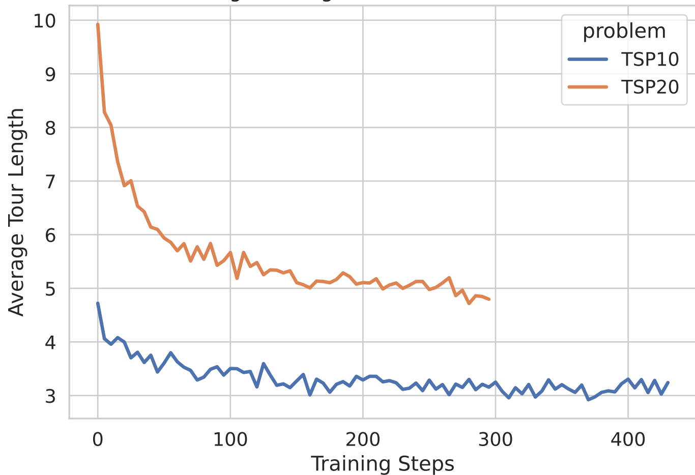
Training Convergence Across Problem Sizes
