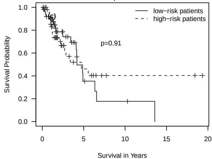
pCox
