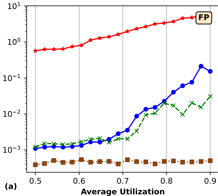
Mean Time to Schedulable Solution (s)
